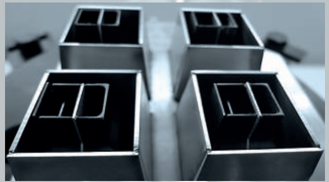
multi-nozzle tool for dip soldering processes
