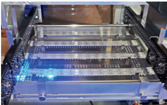
gradient-controlled preheat process
